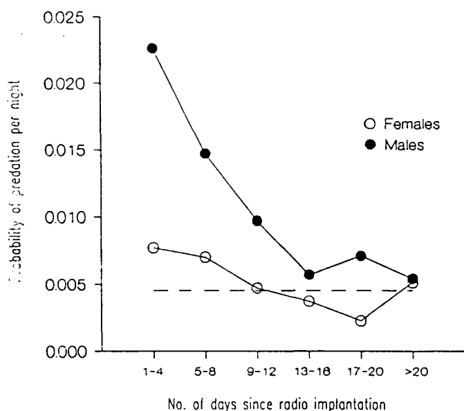
FIG. 1. Predation rates upon radio-implanted kangaroo rats as a function of the victim's sex and of the time elapsed since radio implantation. The figure is based on 52 predation deaths and 337 radio implantations between 1980 and 1991. The broken line represents the estimated predation rate on unimplanted animals (see text).
